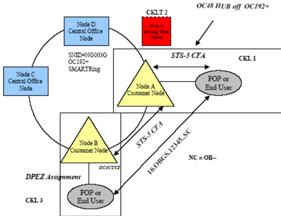
Figure 42. OC192+ SMARTRing Drawing 6a-2
